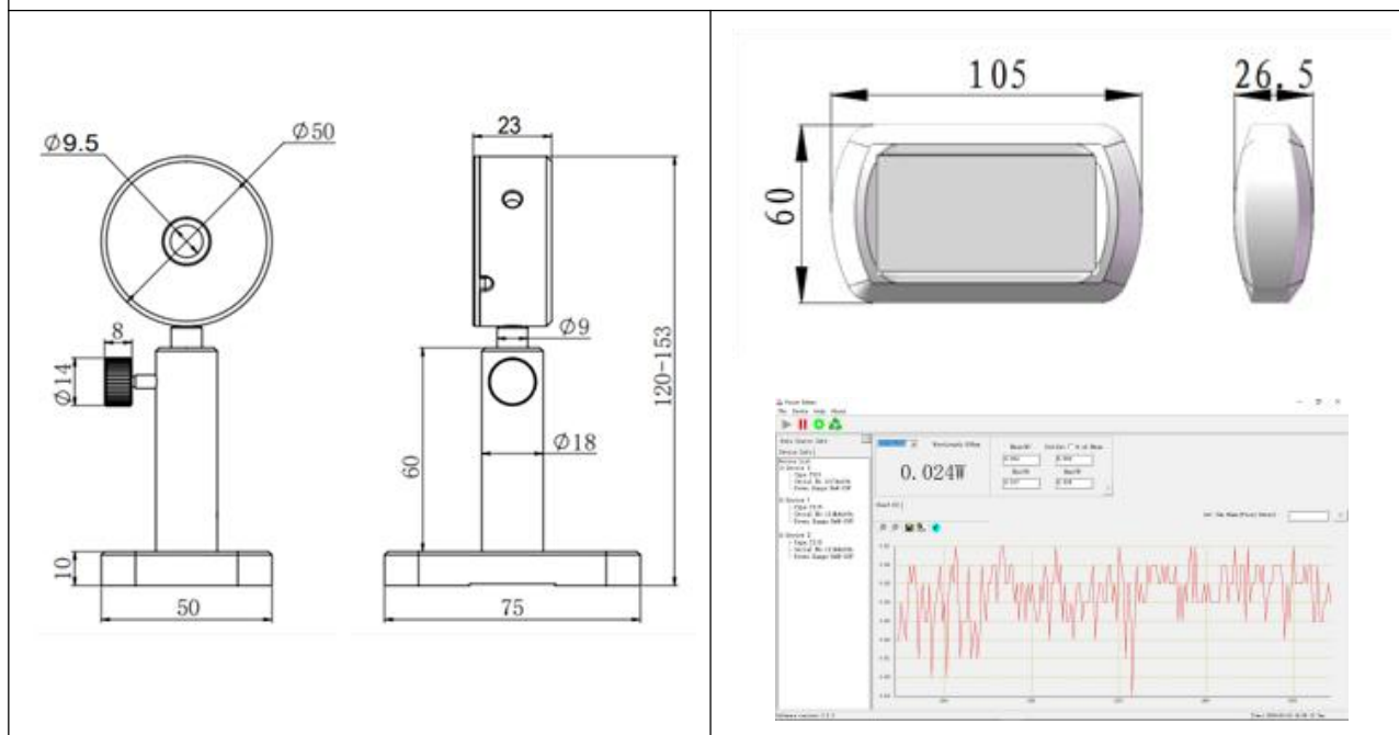
USB Power Meter PD100-350-USB
