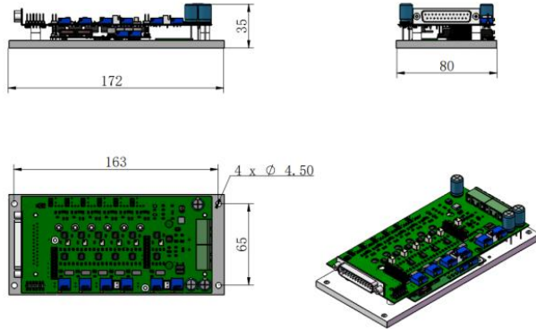
(2 pcs for 520nm and 1 pcs for 455nm) 172 (L)*80 (W)*35 (H) mm 3
