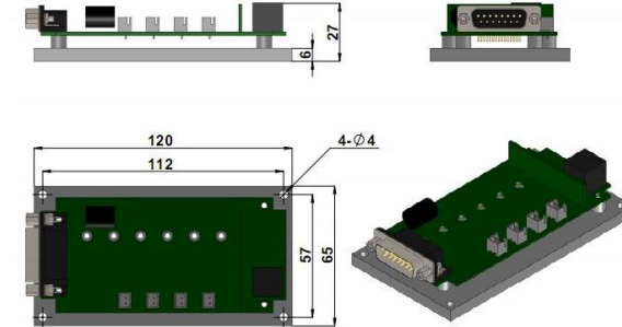
(2 pcs for 635nm) 120 (L)*65 (W)*27 (H) mm 3
