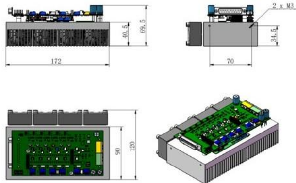
(2 pcs for 520nm and 1 pcs for 455nm) 172 (L)*120 (W)*69.5 (H) mm 3
