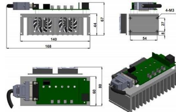
(2 pcs for 635nm) 168 (L)*80 (W)*67 (H) mm 3
