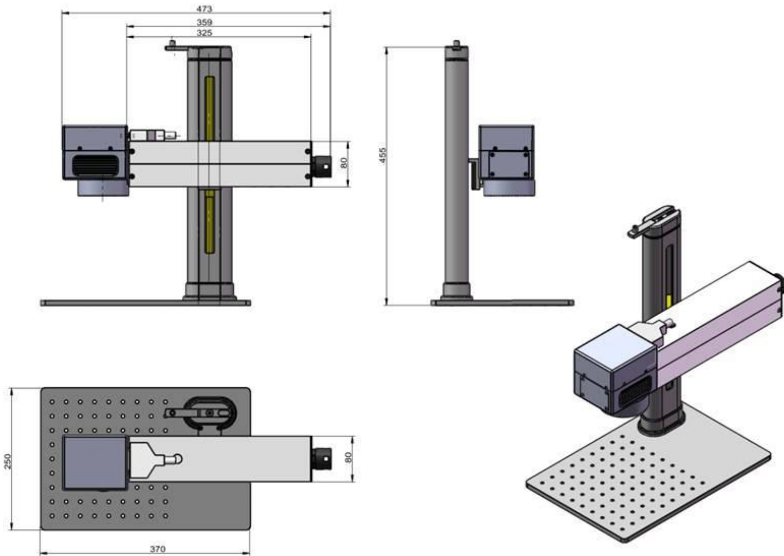
Dimensions of Mini Laser Marking Machine – Laser Head
