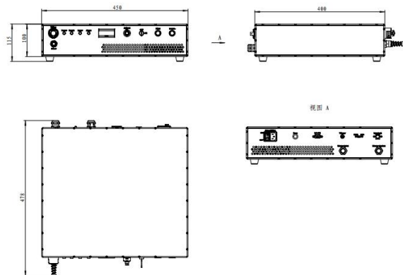
478(L) ×450 (W) ×115 (H) mm 3
