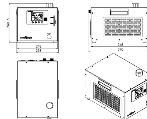
Water Chiller(WCH-580)
