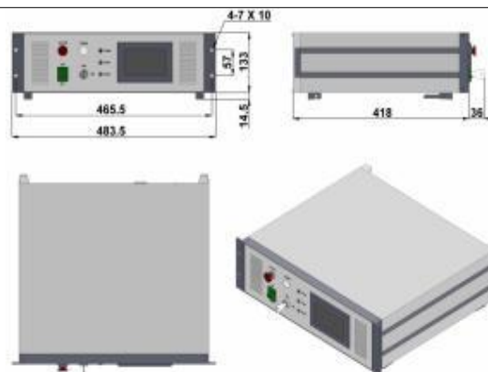
PSU-AOM (3U)
