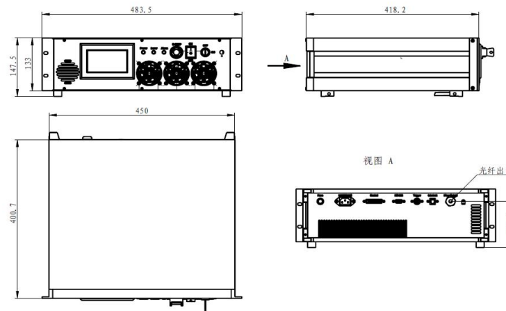
FC-W-450C (Air cooled)
