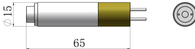
Dimensions of external PCB( 38 \times 14 \times 8 \text{mm}^3 , 3VDC, internal control 750hz frequency)
