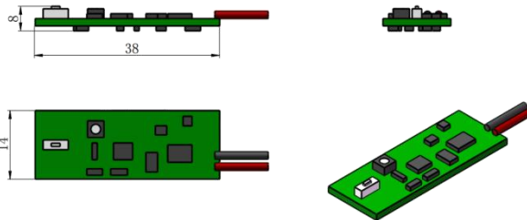
Dimensions of external PCB( 19 \times 15 \times 11.2 \text{mm}^3 , 3VDC)
