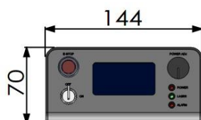
Dimensions of power supply: PSU-A-D (mm)
