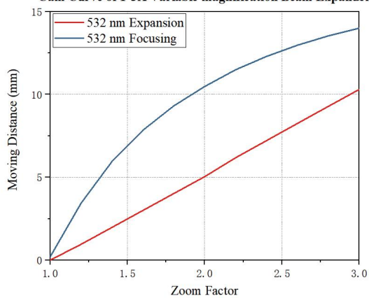
Cam Curve of 1-3X Variable magnification Beam Expander
